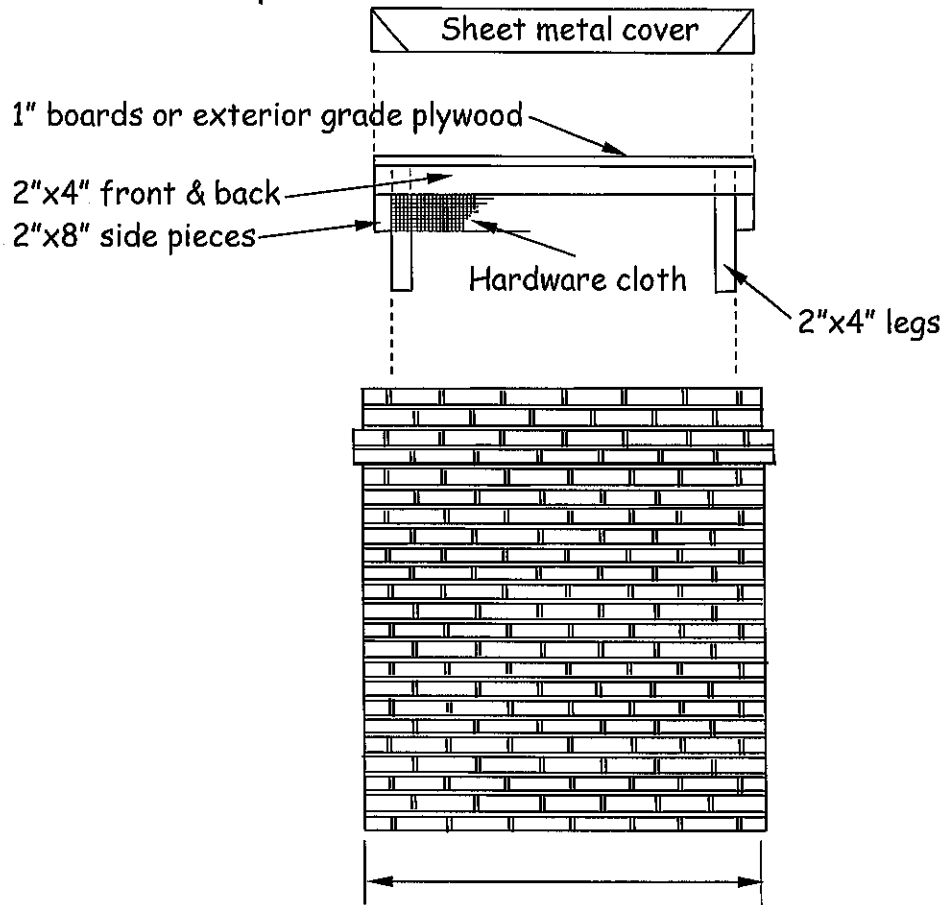
Chimney measures approximately 5'-0" wide by 4'-0" deep
