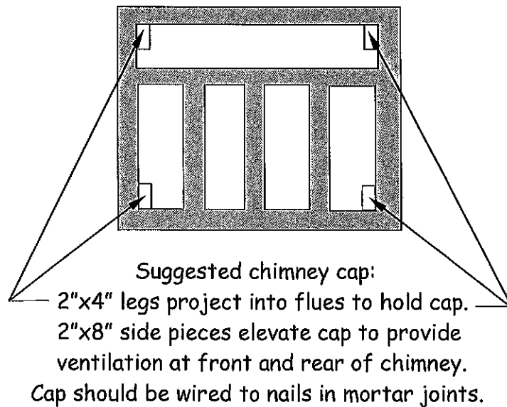
Chimney measures approximately 5'-0" wide by 4'-0" deep
