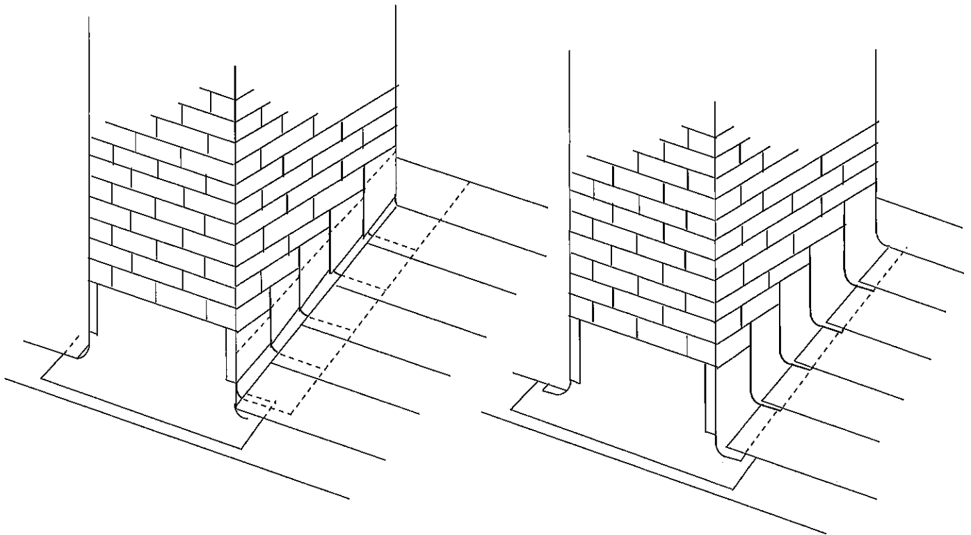
Cap and base flashing The best practice
